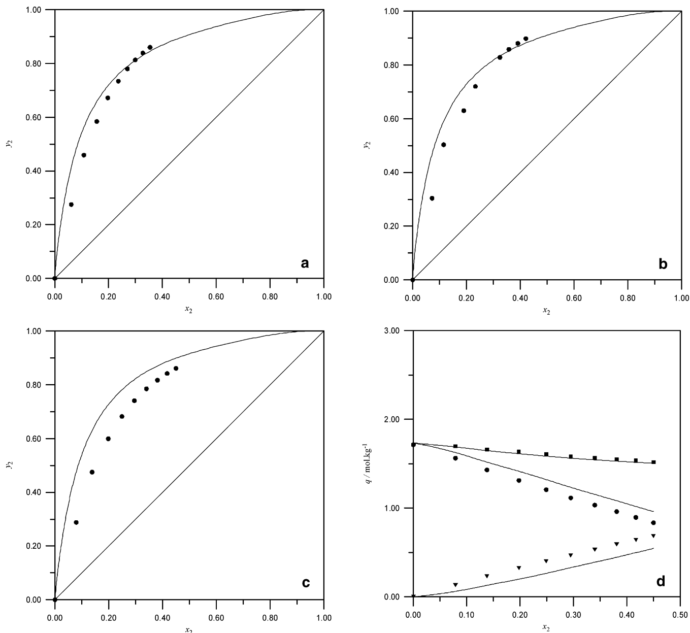
Figure 3. Fit of IAST using Unilan isotherm model to the x - y data for ethane (2) + ethylene (3) (a) at 280 K and 150 kPa, (b) at 280 K and 250 kPa, and (c) at 325 K and 150 kPa. ●, data; y , gas-phase mole fraction; x , adsorbed-phase mole fraction. (d) Fit of IAST using Unilan isotherm model to the x - q data for ethane (2) + ethylene (3) at 325 K and 150 kPa. ▼, methane; ●, ethane; ■, total; x , adsorbed-phase mole fraction; q , amount adsorbed.
