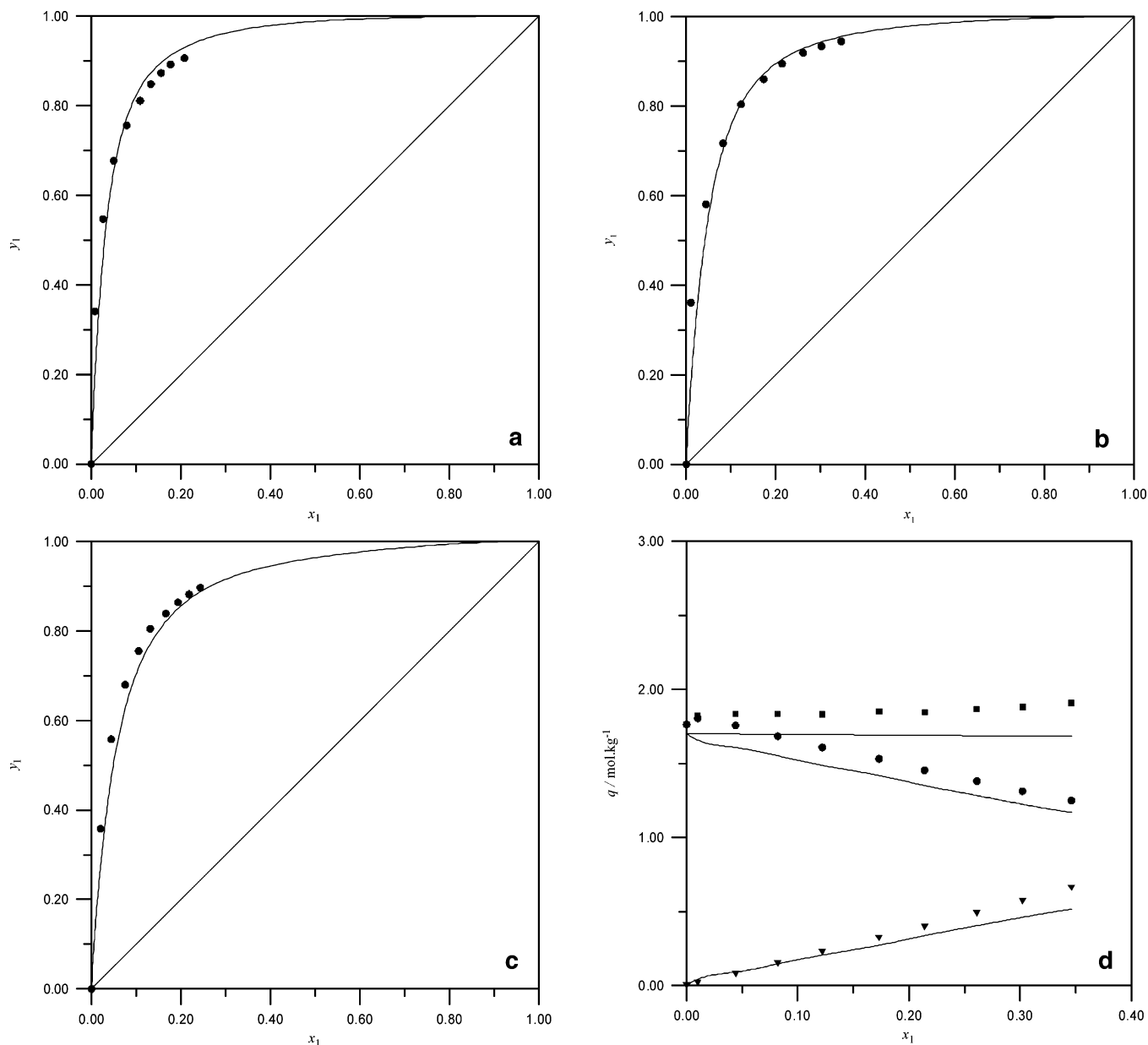
Figure 1. Fit of IAST using Toth isotherm model to the x - y data for methane (1) + ethane (2) (a) at 280 K and 150 kPa, (b) at 280 K and 500 kPa, and (c) at 325 K and 150 kPa. \bullet , data; y , gas-phase mole fraction; x , adsorbed-phase mole fraction. (d) Fit of IAST using Toth isotherm model to the x - q data for methane (1) + ethane (2) at 280 K and 500 kPa. \nabla , methane; \bullet , ethane; \blacksquare , total; x , adsorbed-phase mole fraction; q , amount adsorbed.
