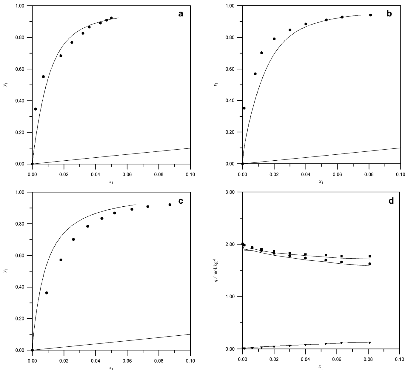
Figure 2. Fit of IAST using Virial isotherm model to the x - y data for methane (1) + ethylene (3) (a) at 280 K and 150 kPa, (b) at 280 K and 250 kPa, and (c) at 325 K and 150 kPa. ●, data; y , gas-phase mole fraction; x , adsorbed-phase mole fraction. (d) Fit of IAST using Virial isotherm model to the x - q data for methane (1) + ethylene (3) at 280 K and 250 kPa. ▼, methane; ●, ethane; ■, total; x , adsorbed-phase mole fraction; q , amount adsorbed.
